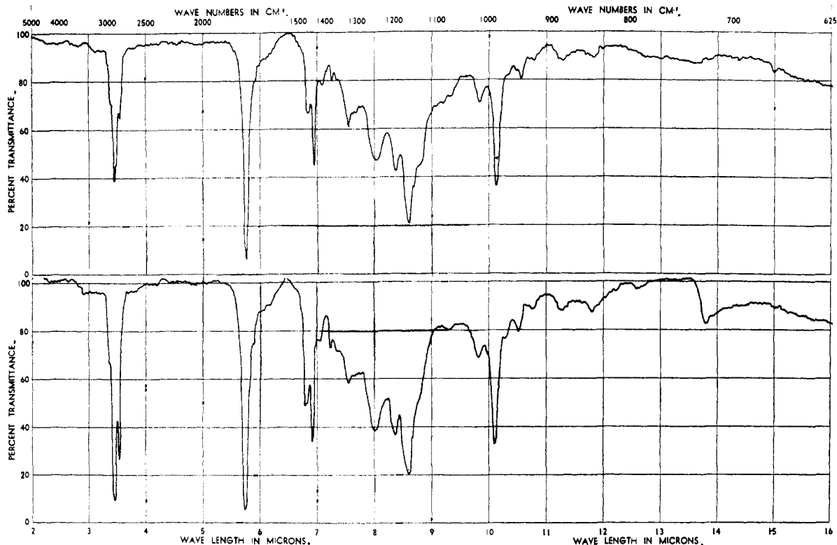
Fig. 2.—Infrared absorption spectra in carbon tetrachloride solution: upper, methyl 3( trans ),5( trans )- n -tridecadienoate; lower, methyl 3( trans ),5( trans )- n -nonadienoate.
