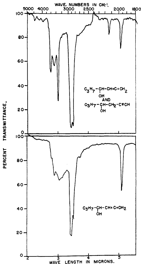
Fig. 4.—Infrared absorption spectra in carbon tetrachloride solution: upper, mixture of allenic and acetylenic alcohols from the Reformatsky reaction of butyraldehyde and zinc propargyl bromide; lower, allenic component from the above reaction products.
